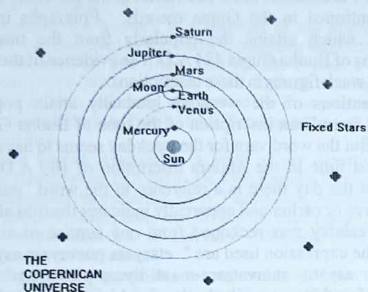
Fig. A1.1 The Copernican Universe
